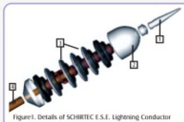
Figure1. Details of SCHIRTEC E.S.E. Lightning Conductor
